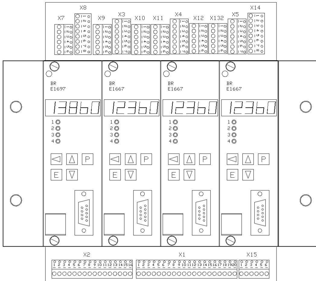
Figure 8: Position of terminal blocks with version E16A352 (shown is version E16A346)
